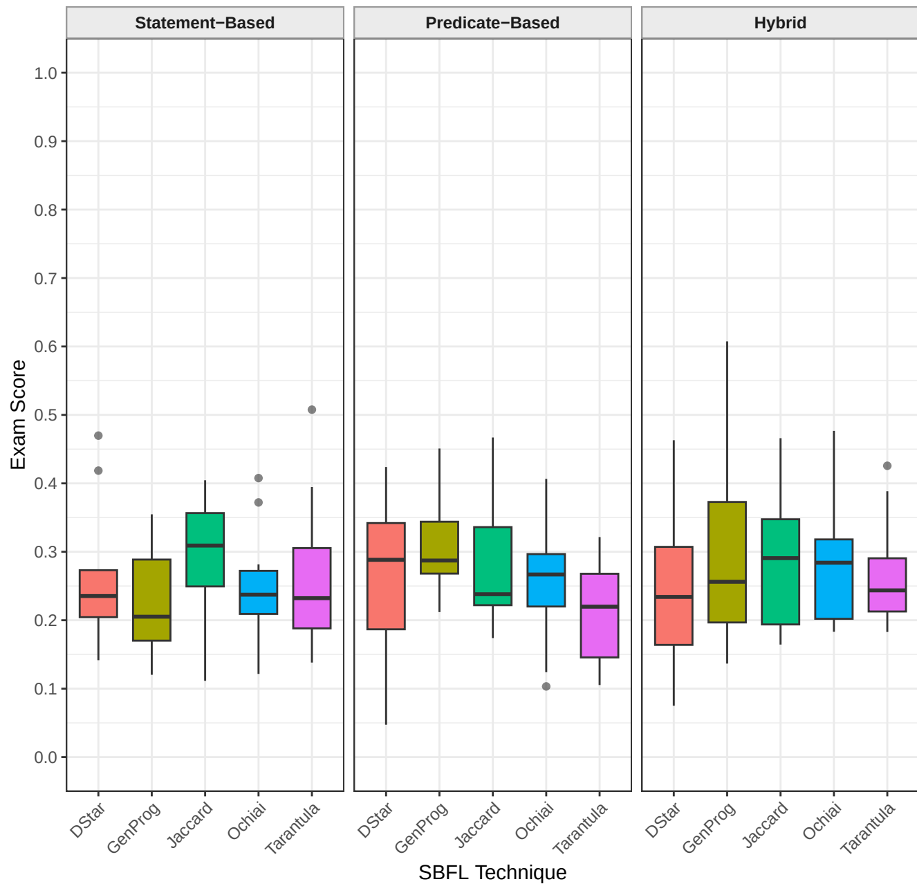
Figure 1: Exam scores under different program elements and different SBFL techniques
