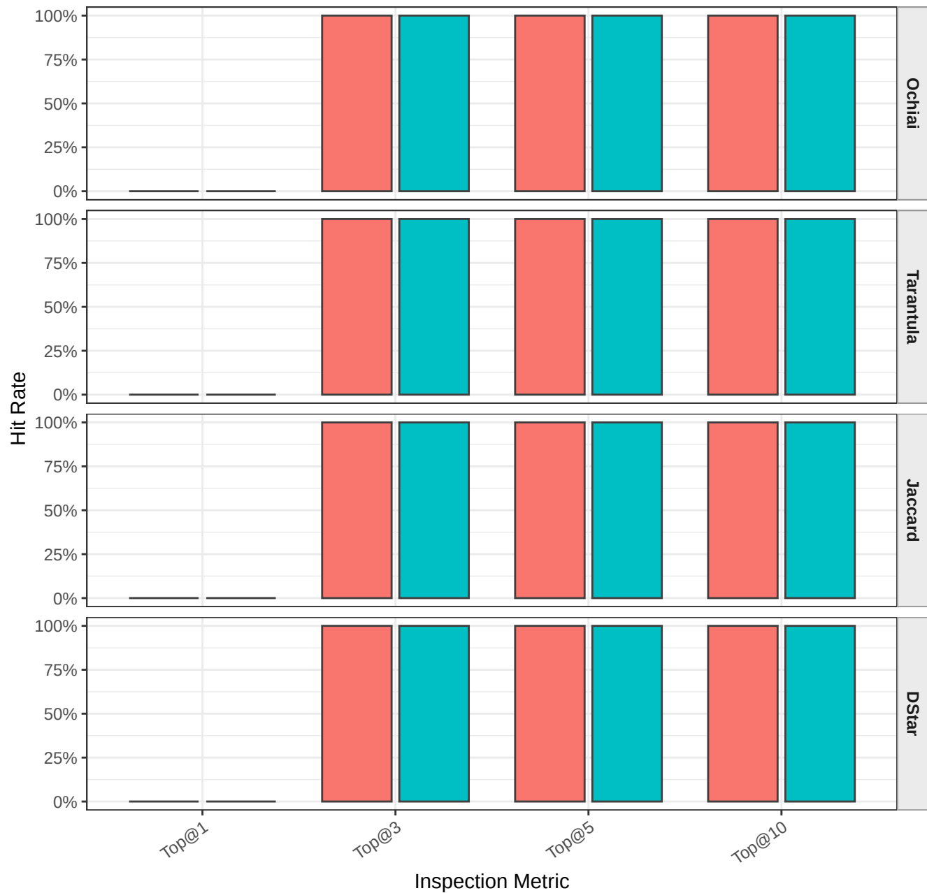
Baseline vs Weighted HDD-LOC: Top-N Inspection Metrics
