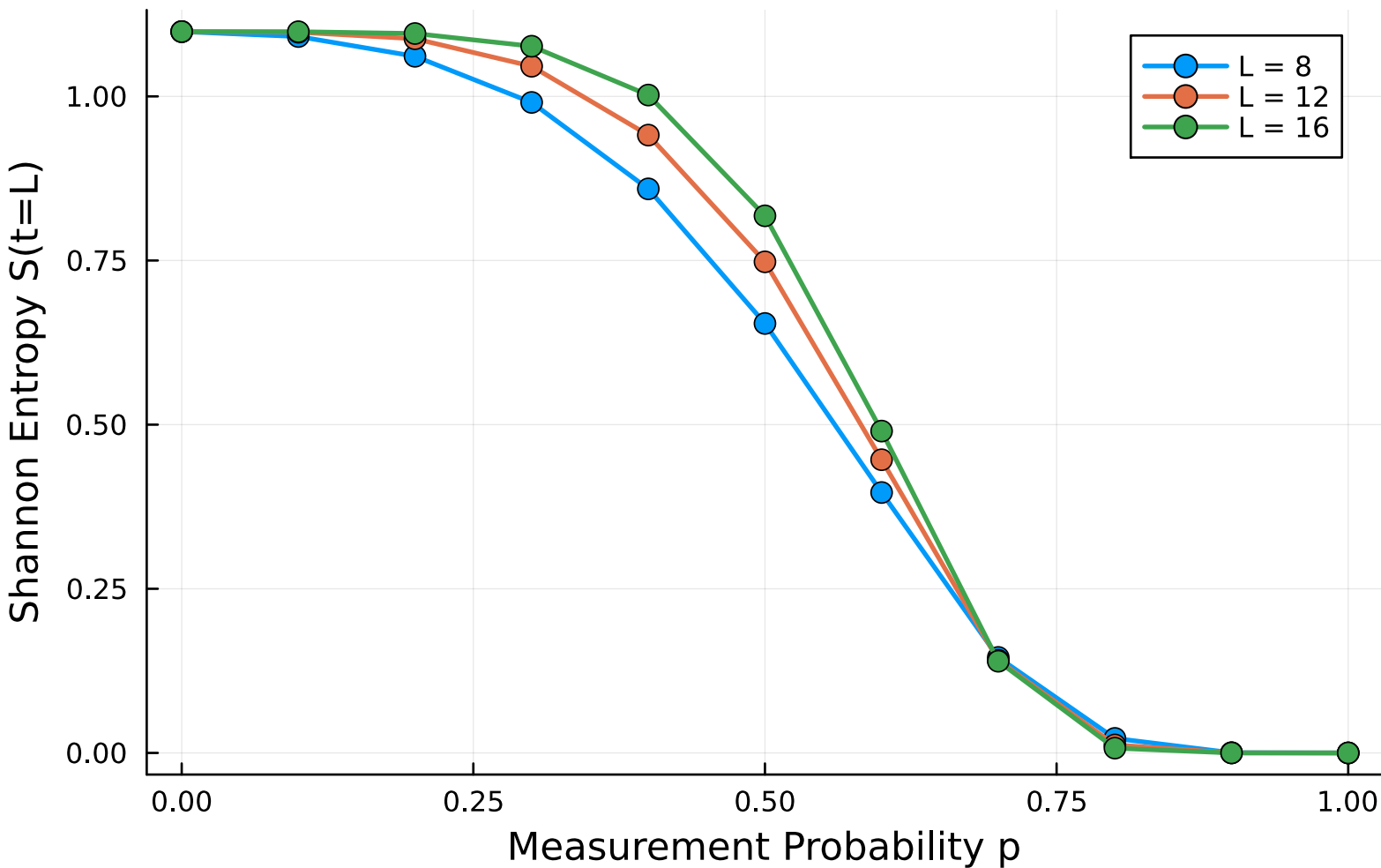
Shannon Entropy at t = L vs Measurement Probability
