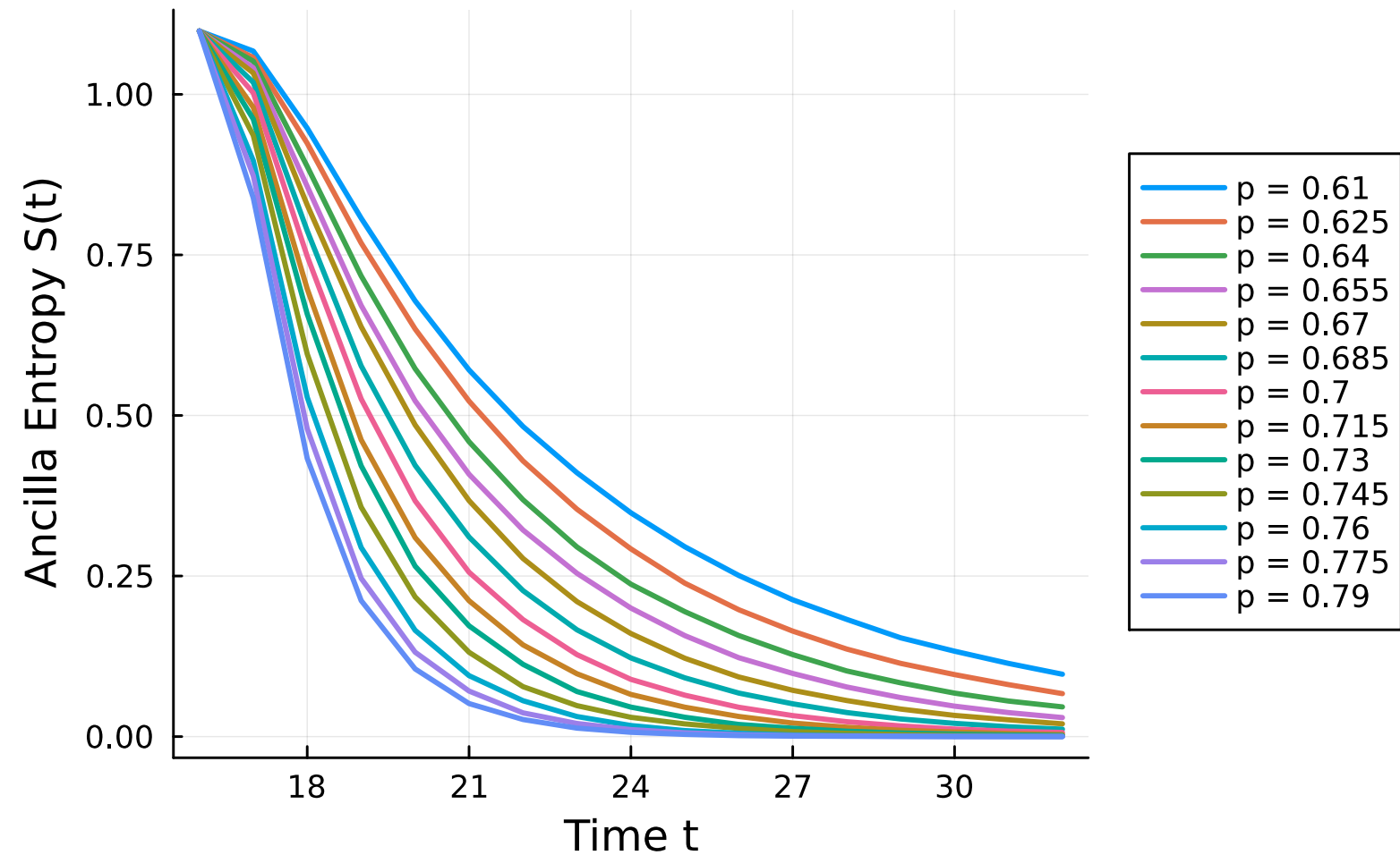
Ancilla Entropy ( L = 16 , t: T \rightarrow 2T )
