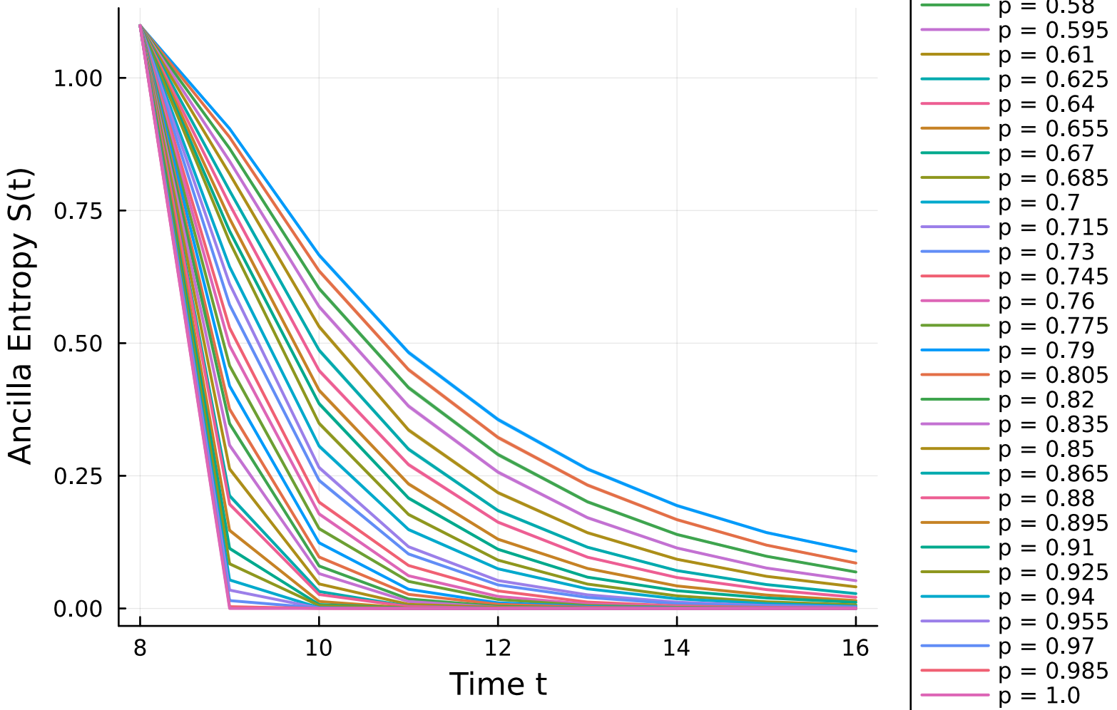
Ancilla Entropy Evolution (L = 8, t: T → 2T)
