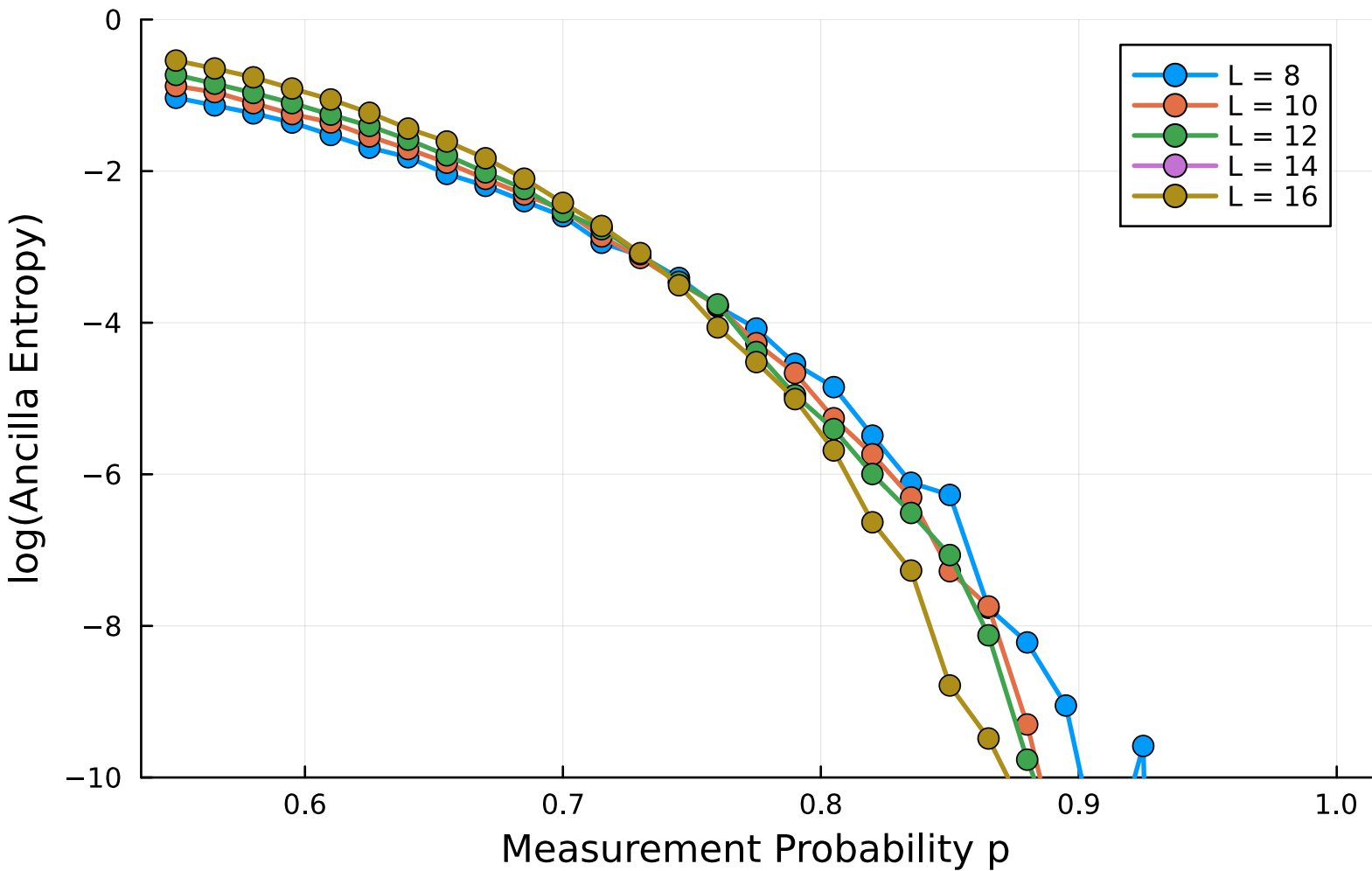
Ancilla Entropy at t = 3L/2 vs Measurement Probability
