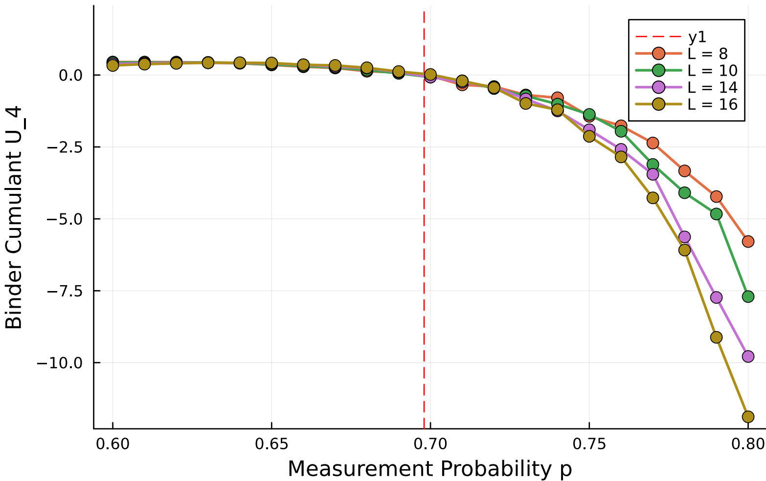
Ensemble Binder Cumulant U_4 at t = 2L
