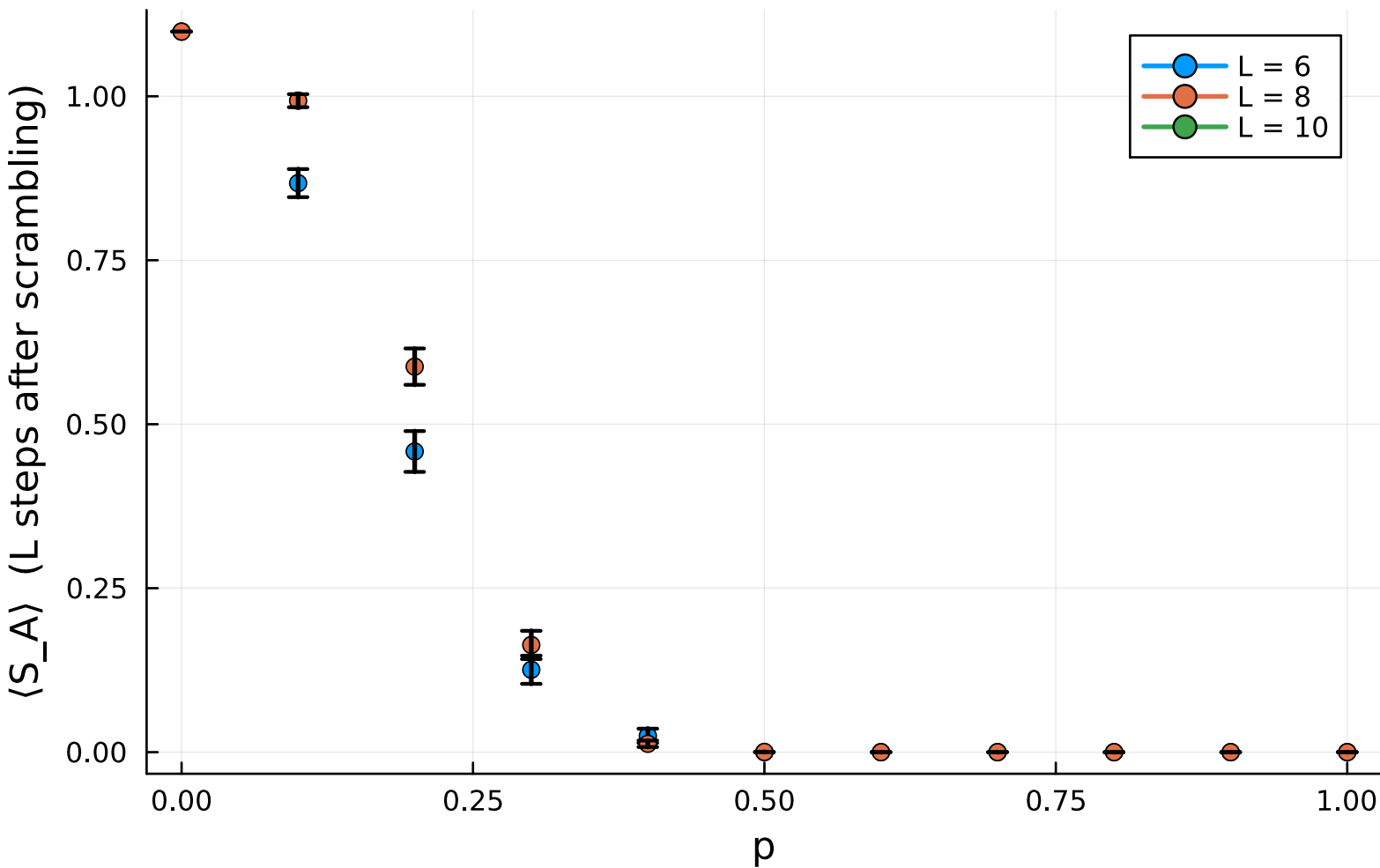
Ancilla entropy L steps post-scramble vs p
