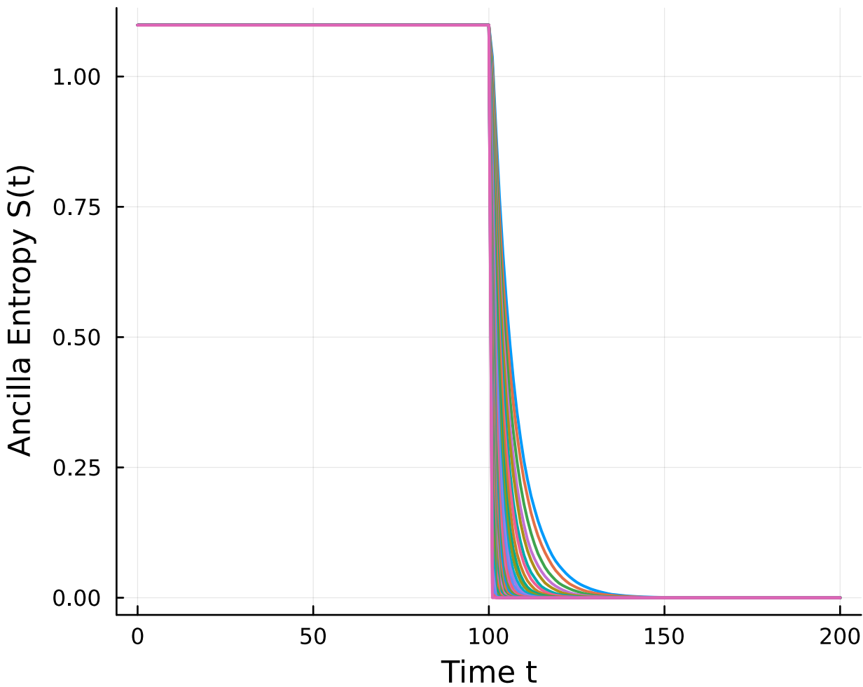
Ancilla Entropy Evolution (L = 10)
