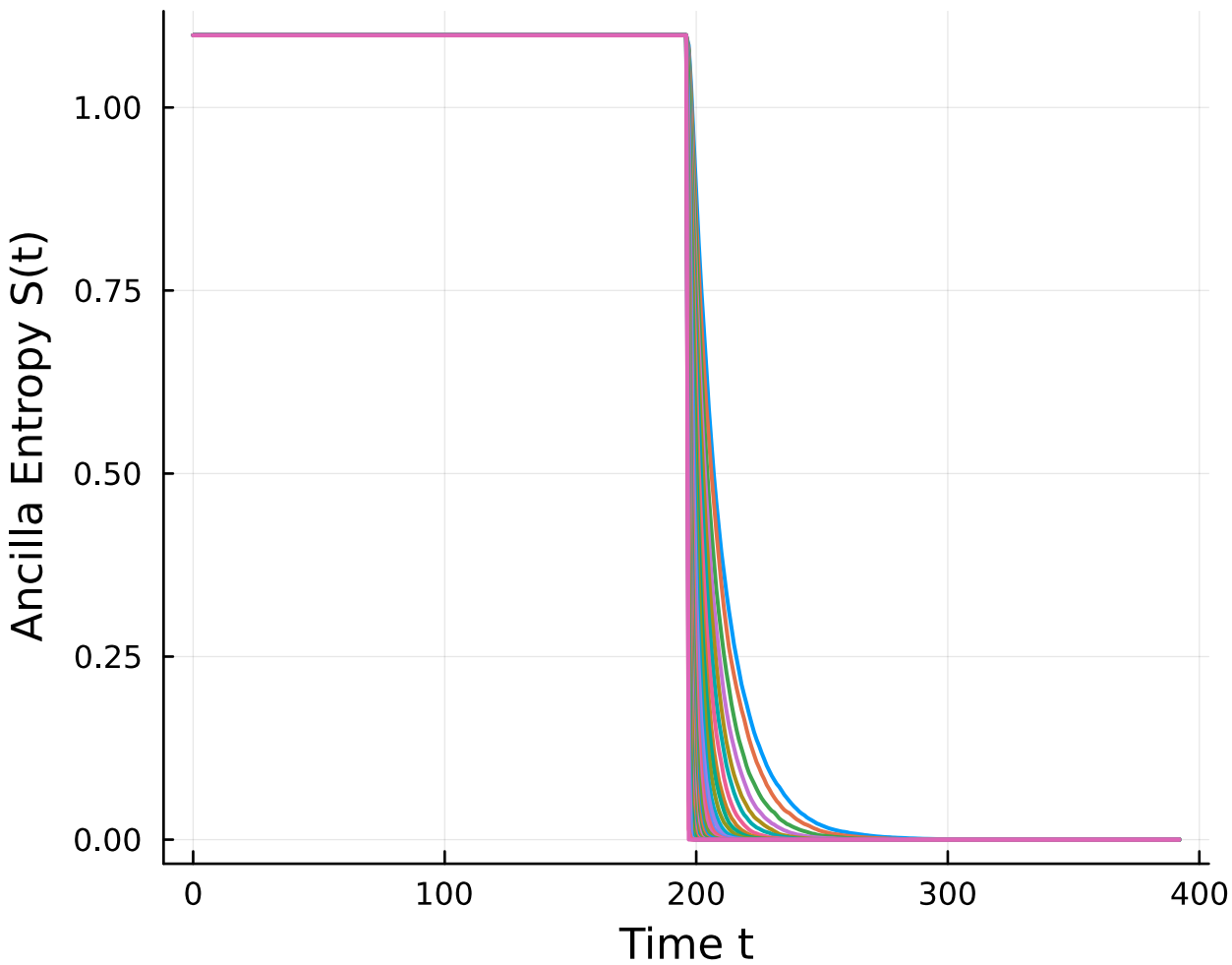
Ancilla Entropy Evolution (L = 14)
