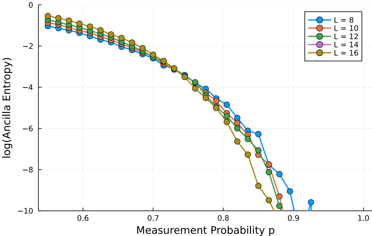
Ancilla Entropy at t = L/2 vs Measurement Probability
