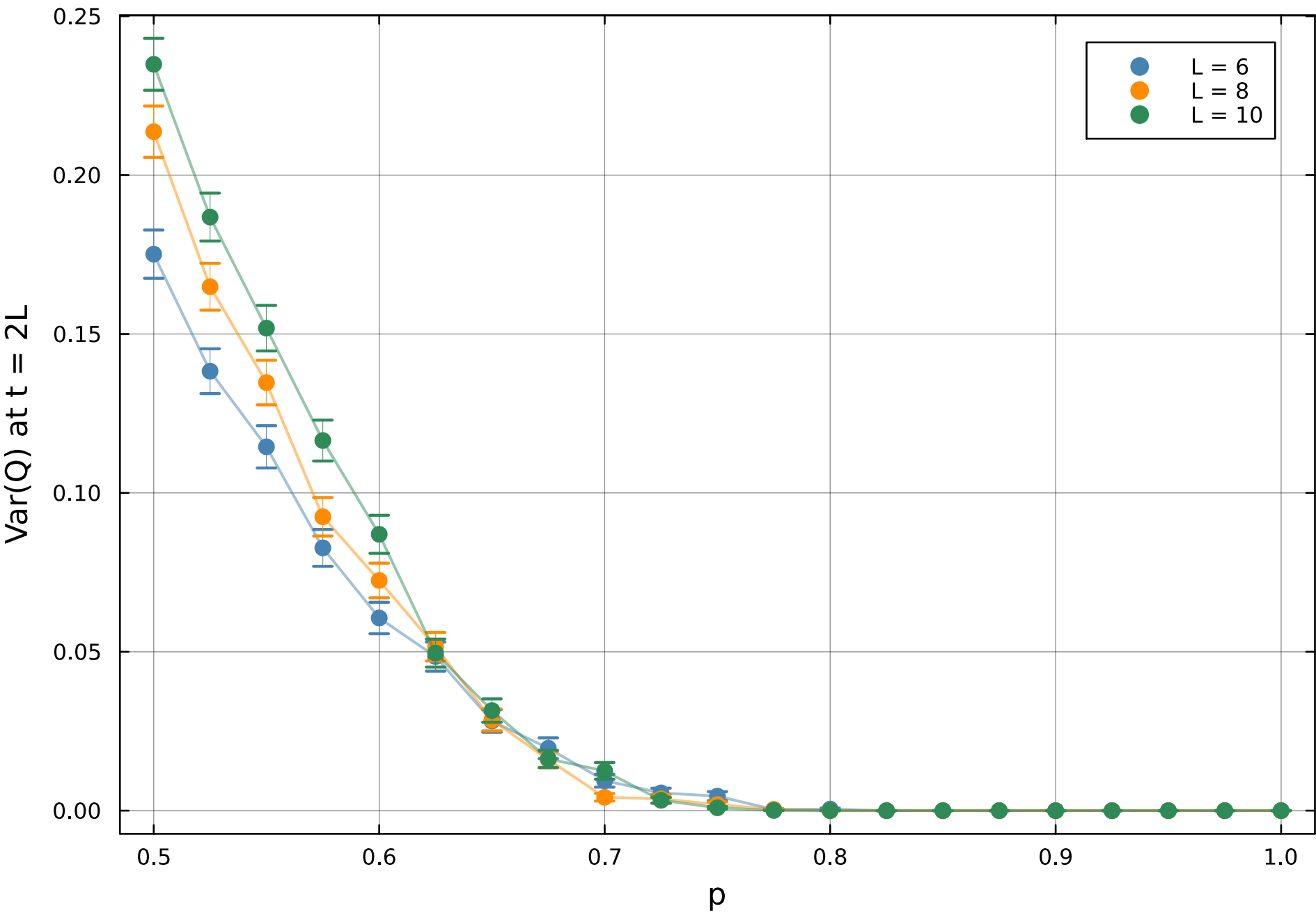
Z_3 charge sharpening: \text{Var}(Q) vs p
