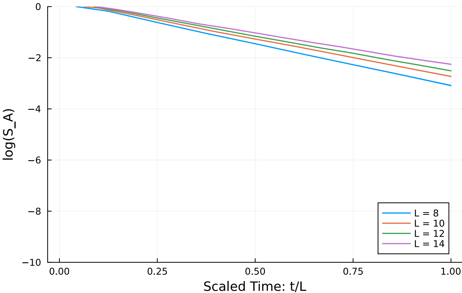
Scaled Log Entropy Evolution ( p = 0.600000 )
