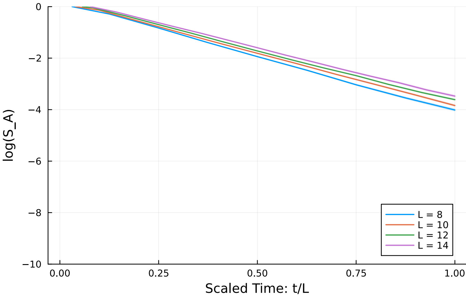
Scaled Log Entropy Evolution ( p = 0.650000 )
