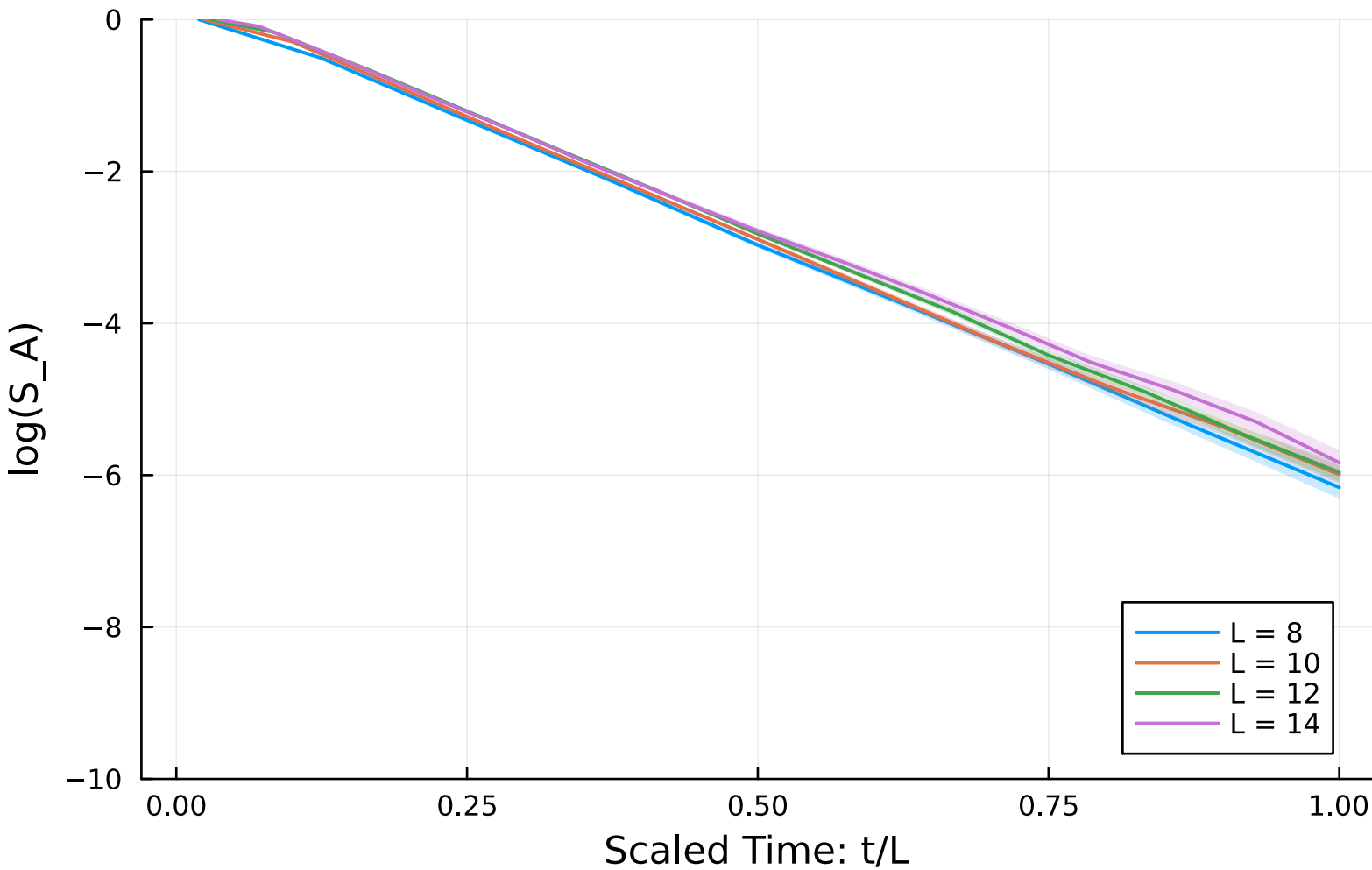
Scaled Log Entropy Evolution ( p = 0.716667 )
