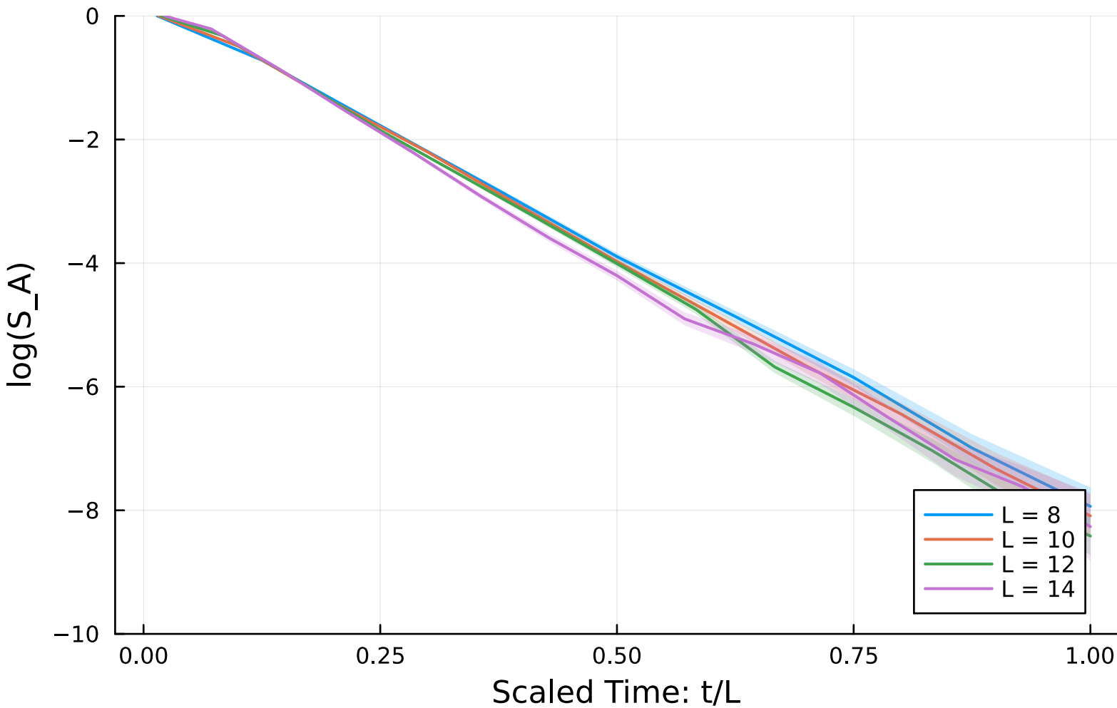
Scaled Log Entropy Evolution ( p = 0.766667 )
