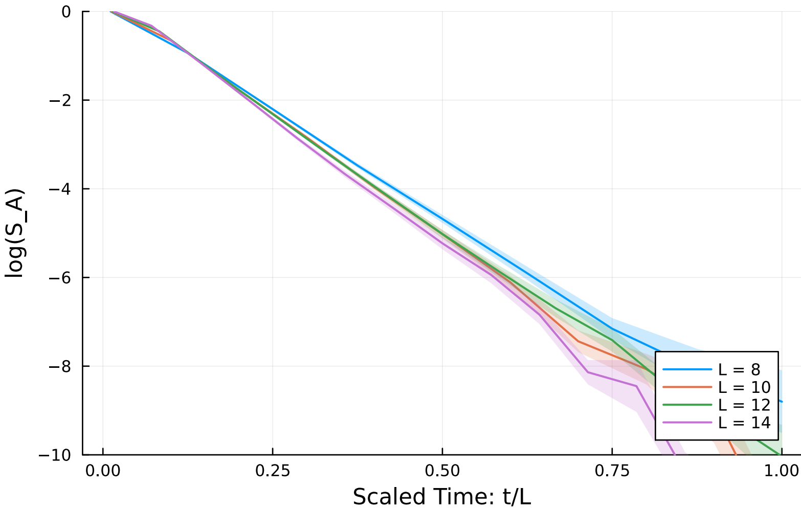
Scaled Log Entropy Evolution ( p = 0.800000 )
