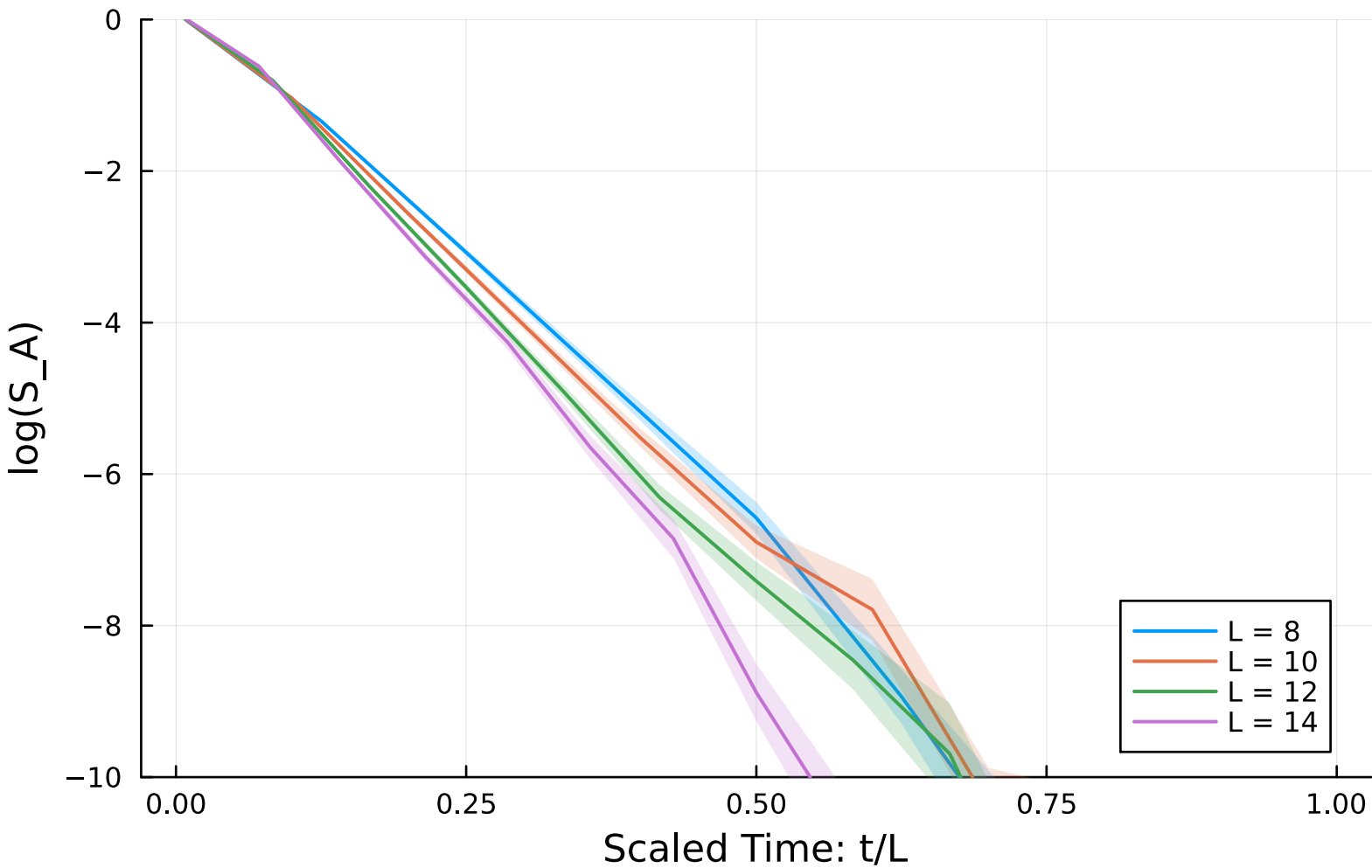
Scaled Log Entropy Evolution ( p = 0.850000 )
