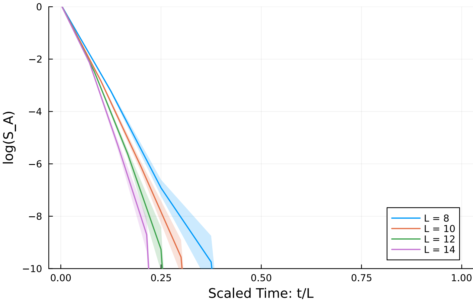
Scaled Log Entropy Evolution ( p = 0.950000 )
