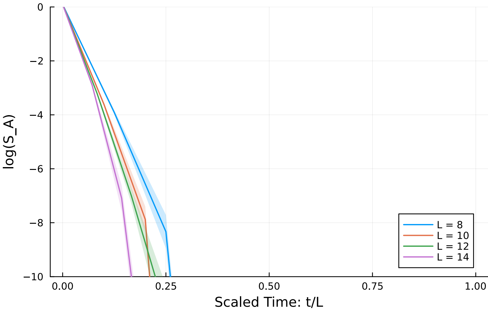
Scaled Log Entropy Evolution ( p = 0.966667 )
