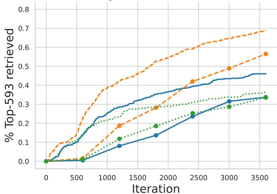
Surrogate = Random Forest
