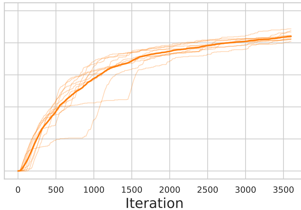
MolFormer
