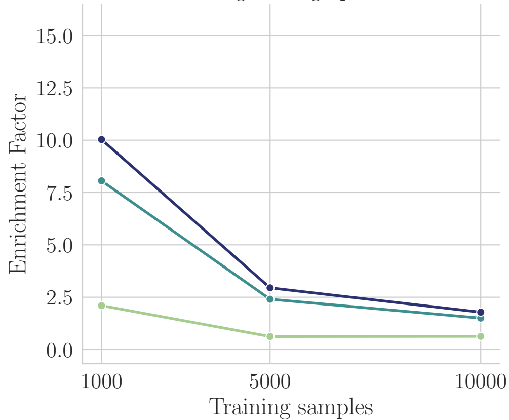
Morgan Fingerprint
