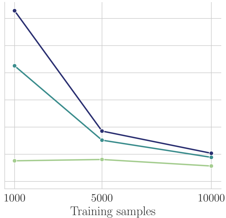
ChemBERTa-2
