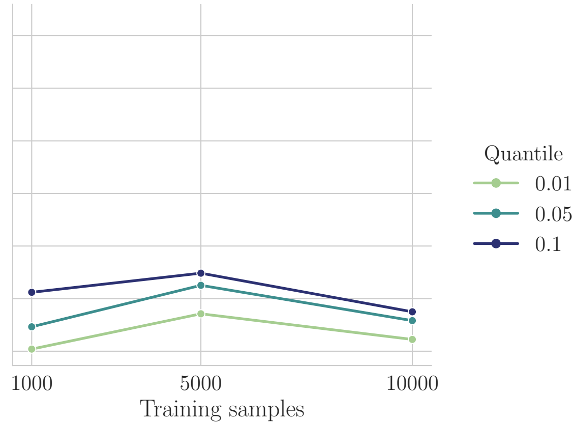
MolFormer
