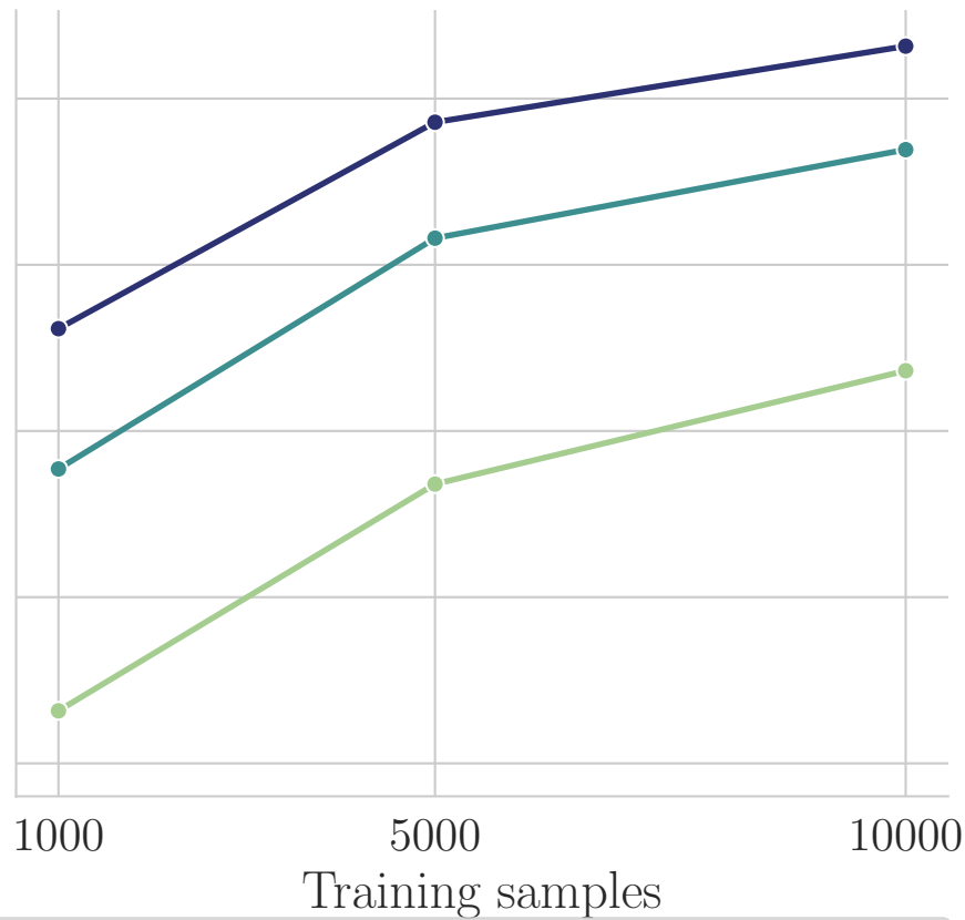
ChemBERTa-2
