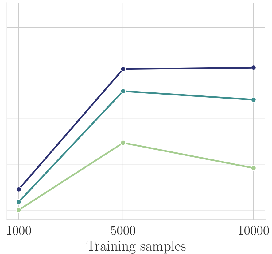
MolFormer
