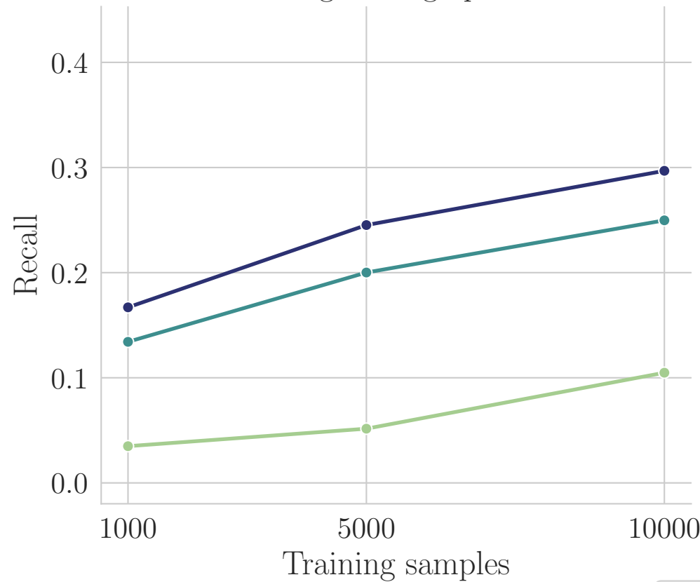
Morgan Fingerprint
