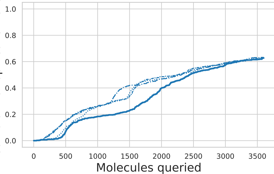
ChemBERTa-2
