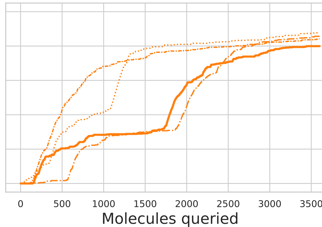
MolFormer
