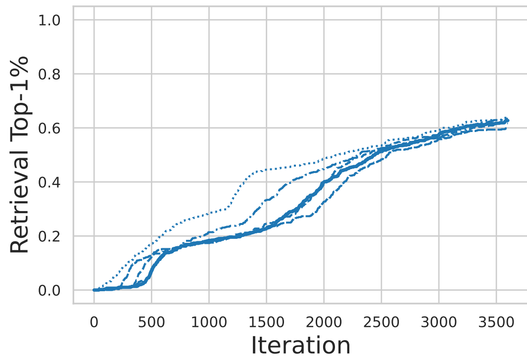
ChemBERTa-2
