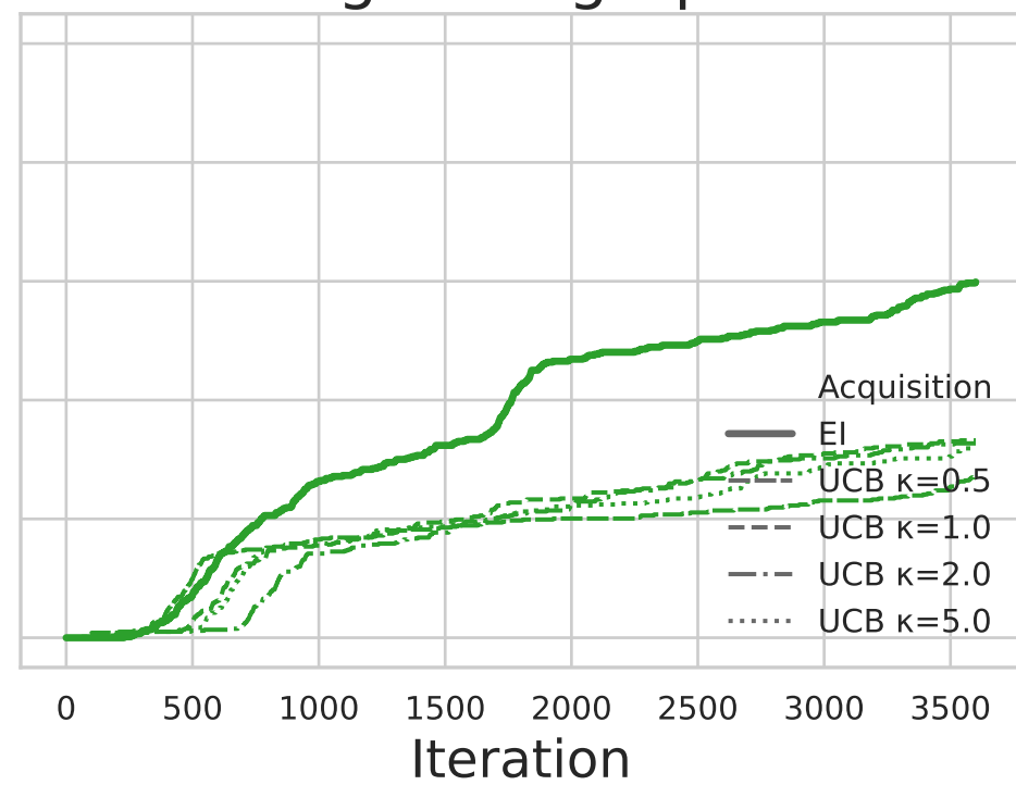
Morgan Fingerprint
