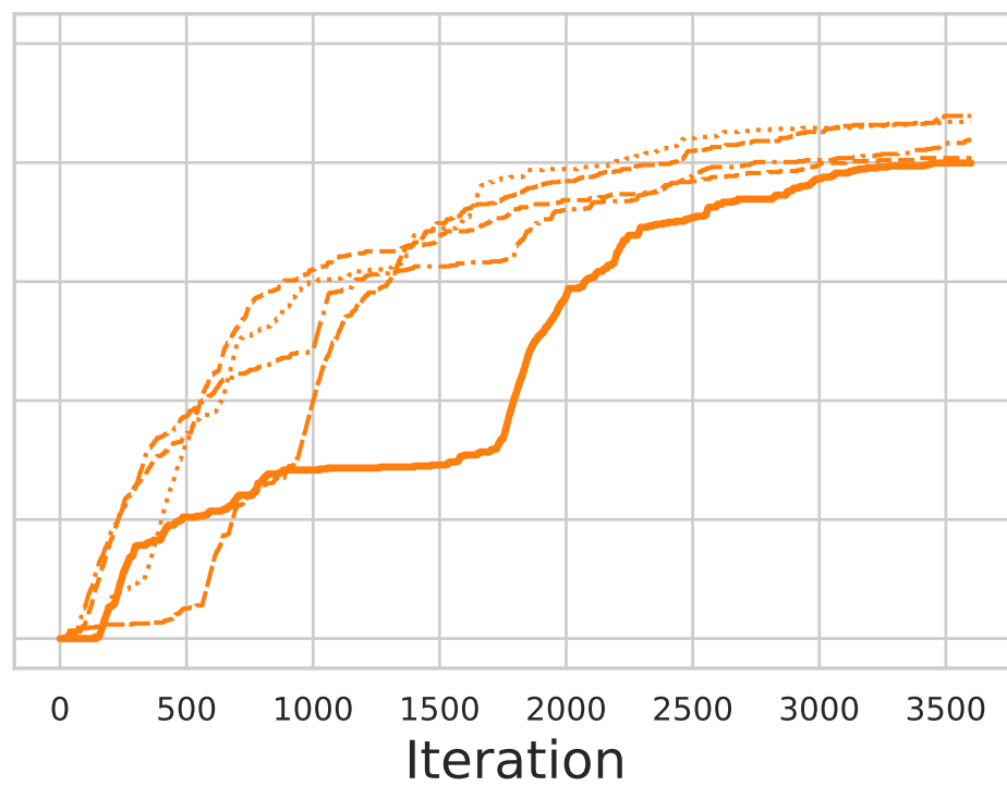
MolFormer
