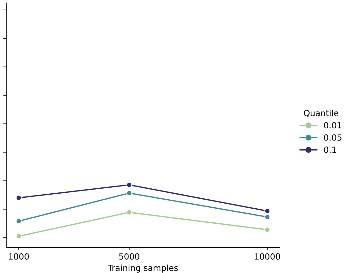
MolFormer
