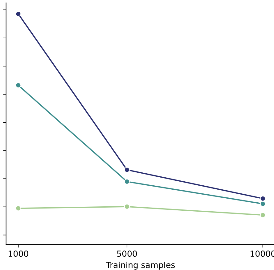
ChemBERTa-2
