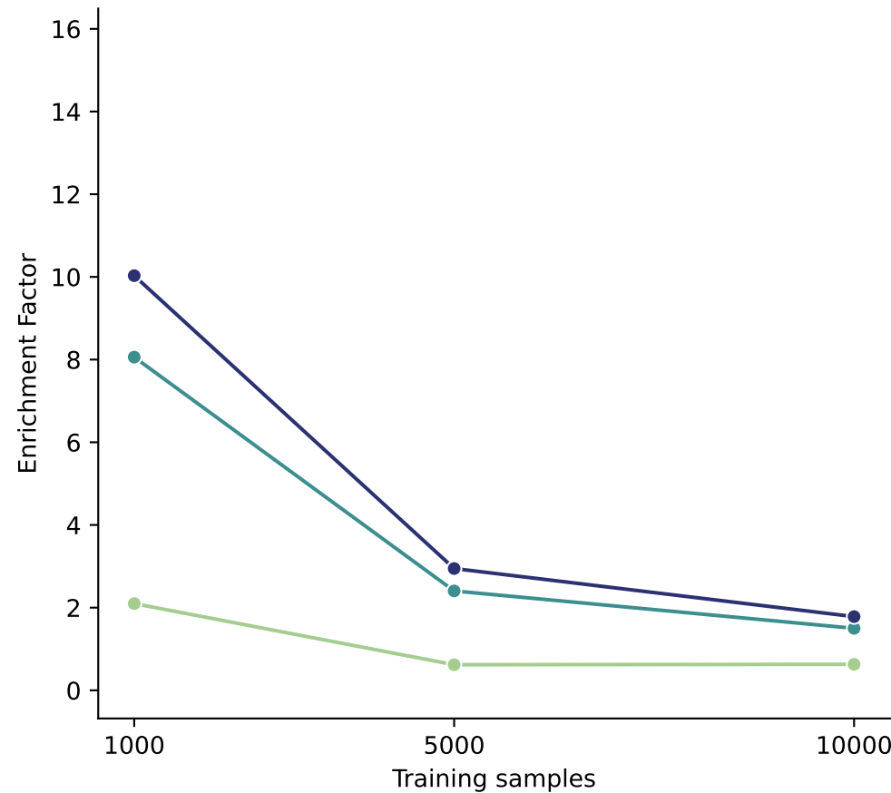
Morgan Fingerprint
