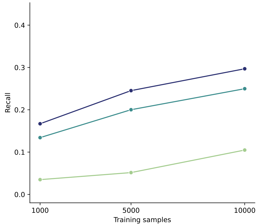
Morgan Fingerprint
