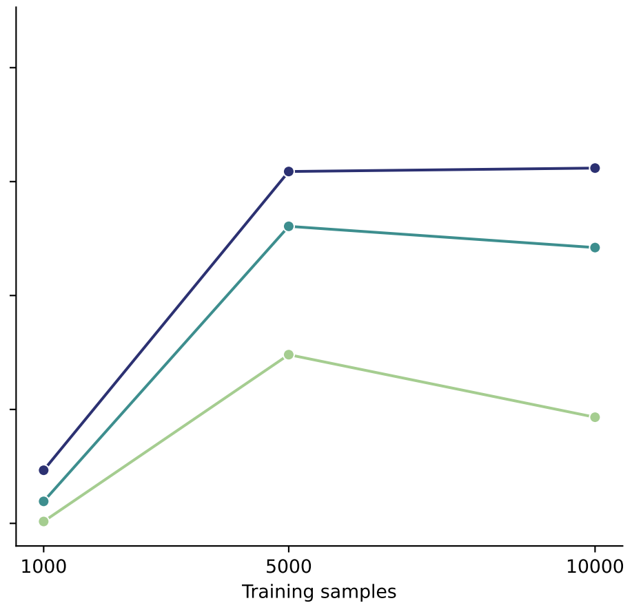
MolFormer
