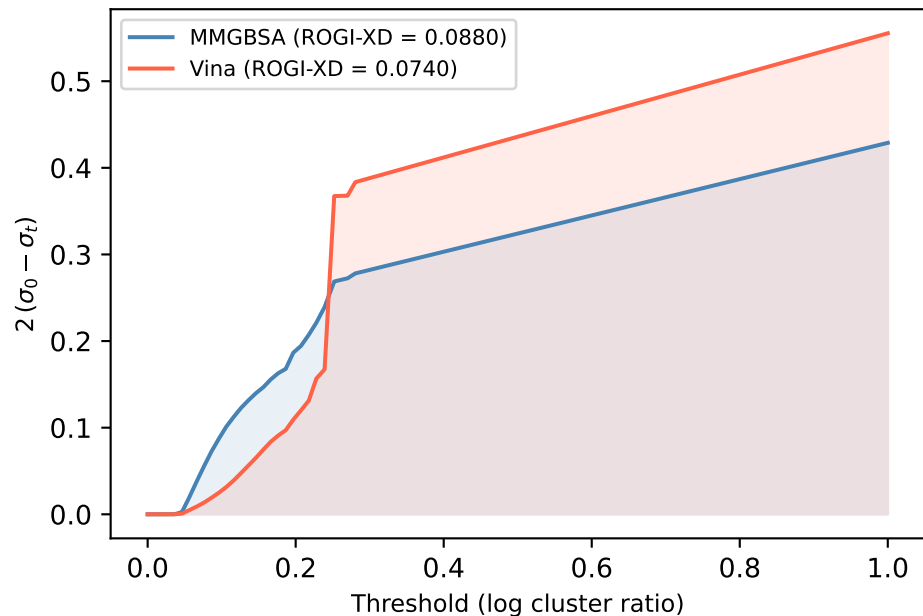
ROGI-XD
