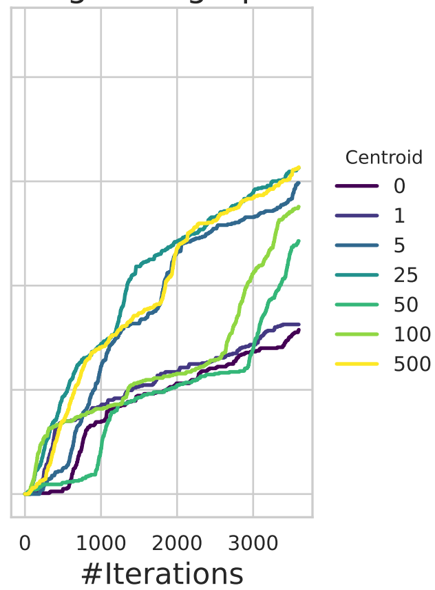
Morgan Fingerprint
