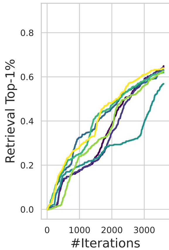
ChemBERTa-2
