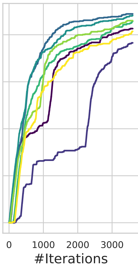
MolFormer
