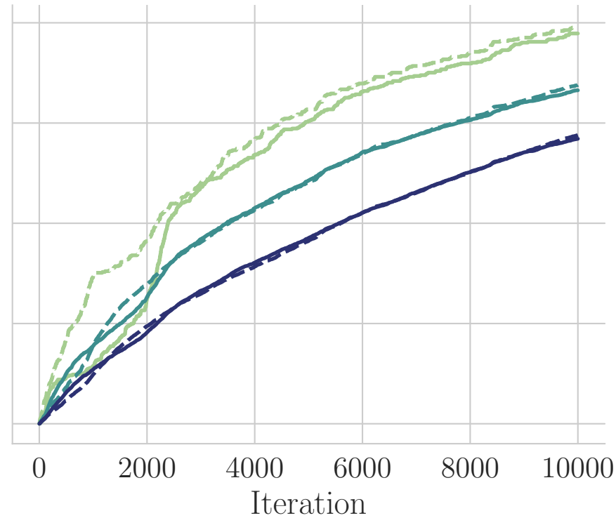
MolFormer
