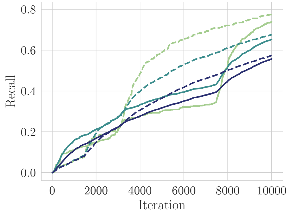
Morgan Fingerprint
