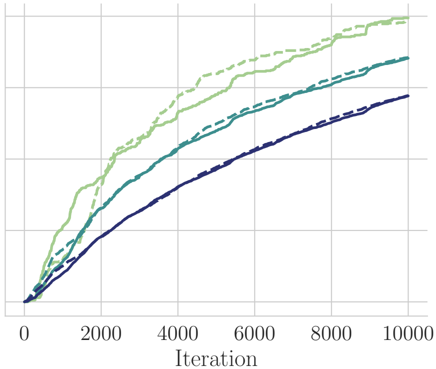
ChemBERTa-2
