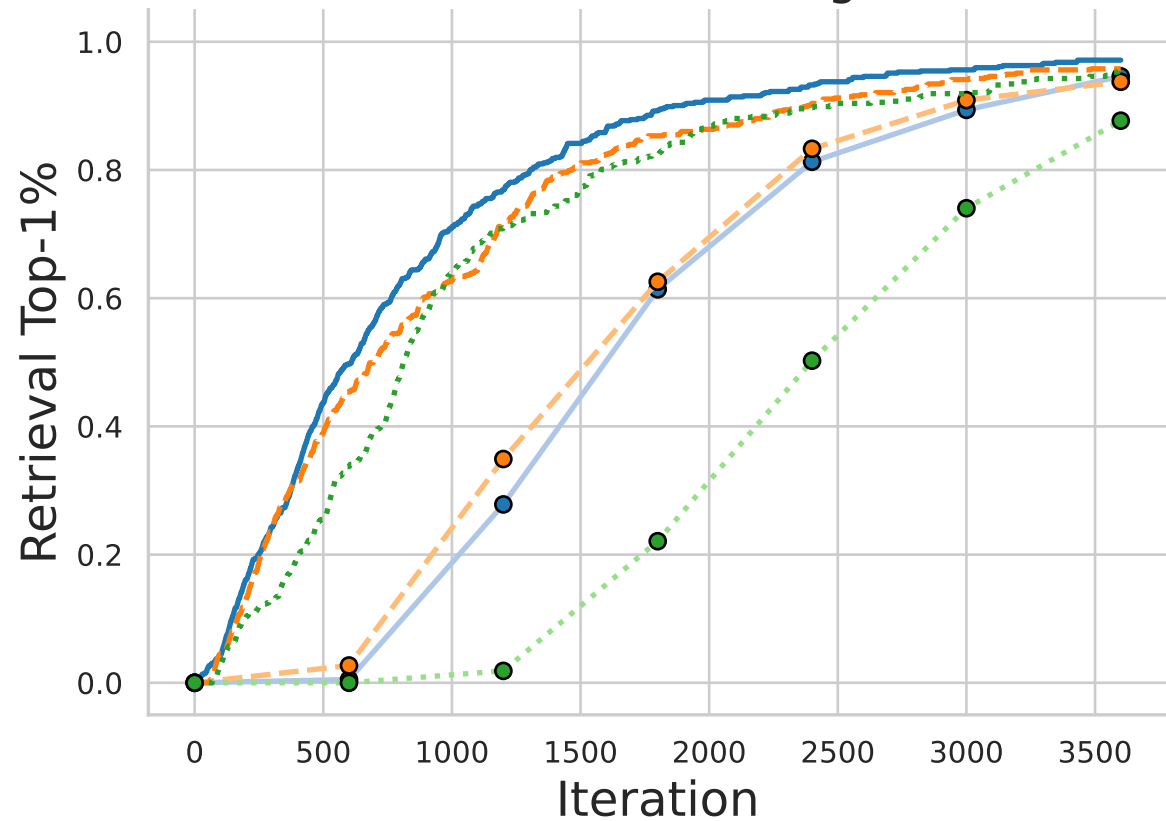
Score = Docking
