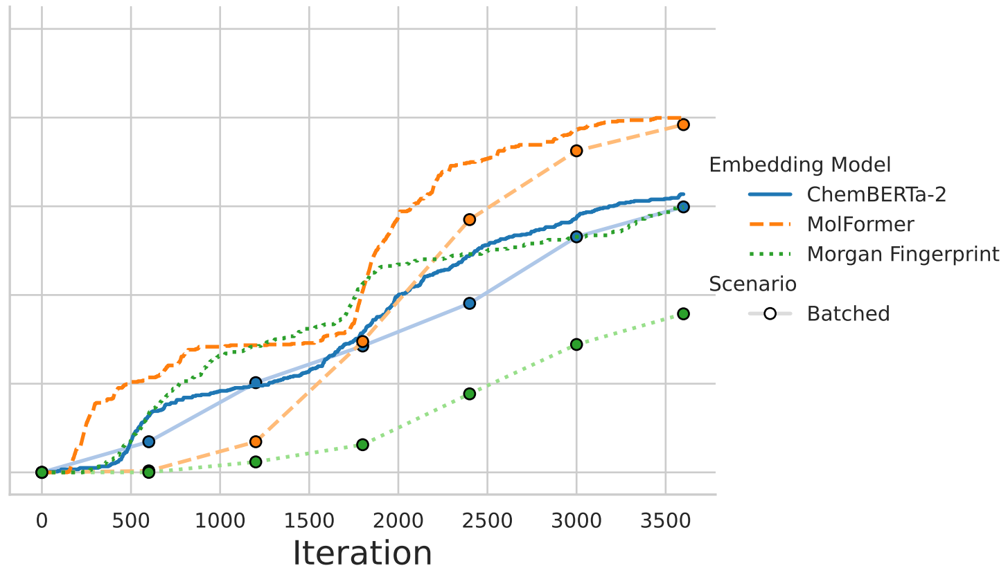
Score = MMGBSA
