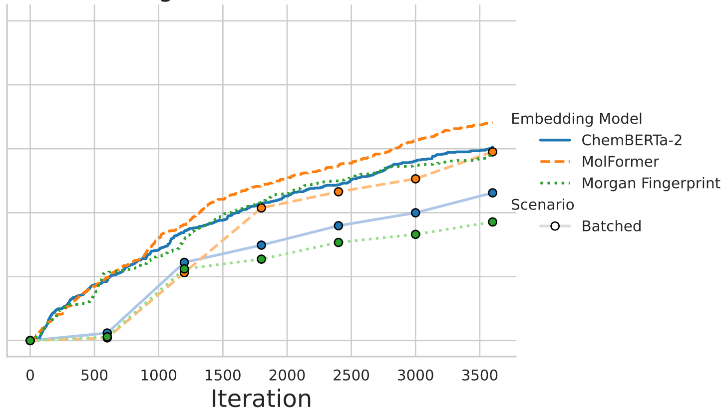
Surrogate = Random Forest
