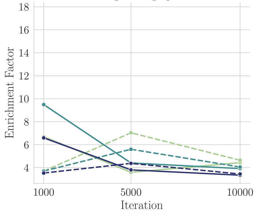
Morgan Fingerprint
