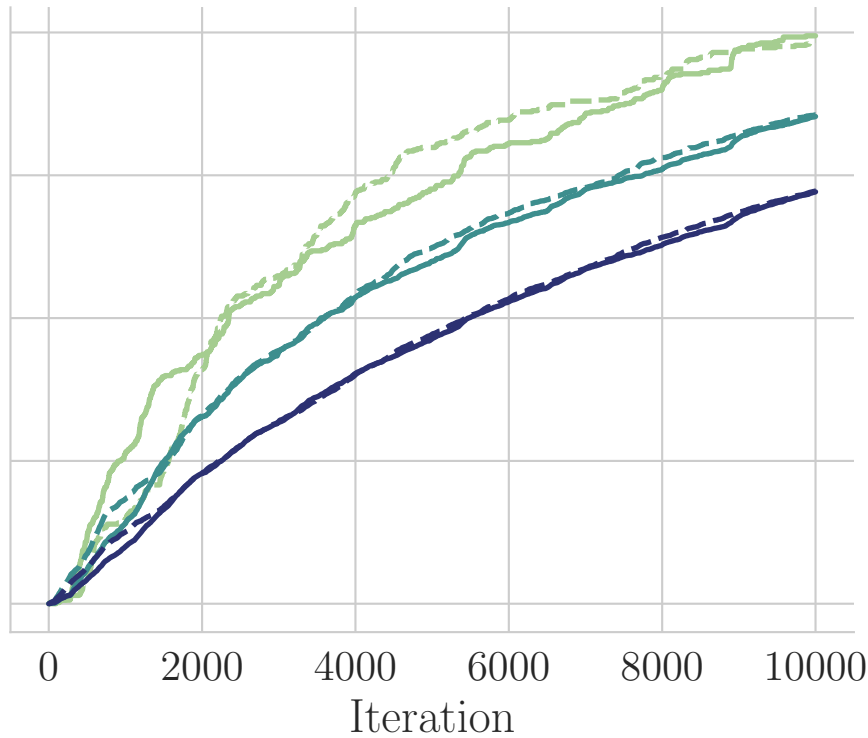
ChemBERTa-2
