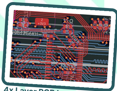
4x Layer PCB based on the STM32H7 with SDRAM
