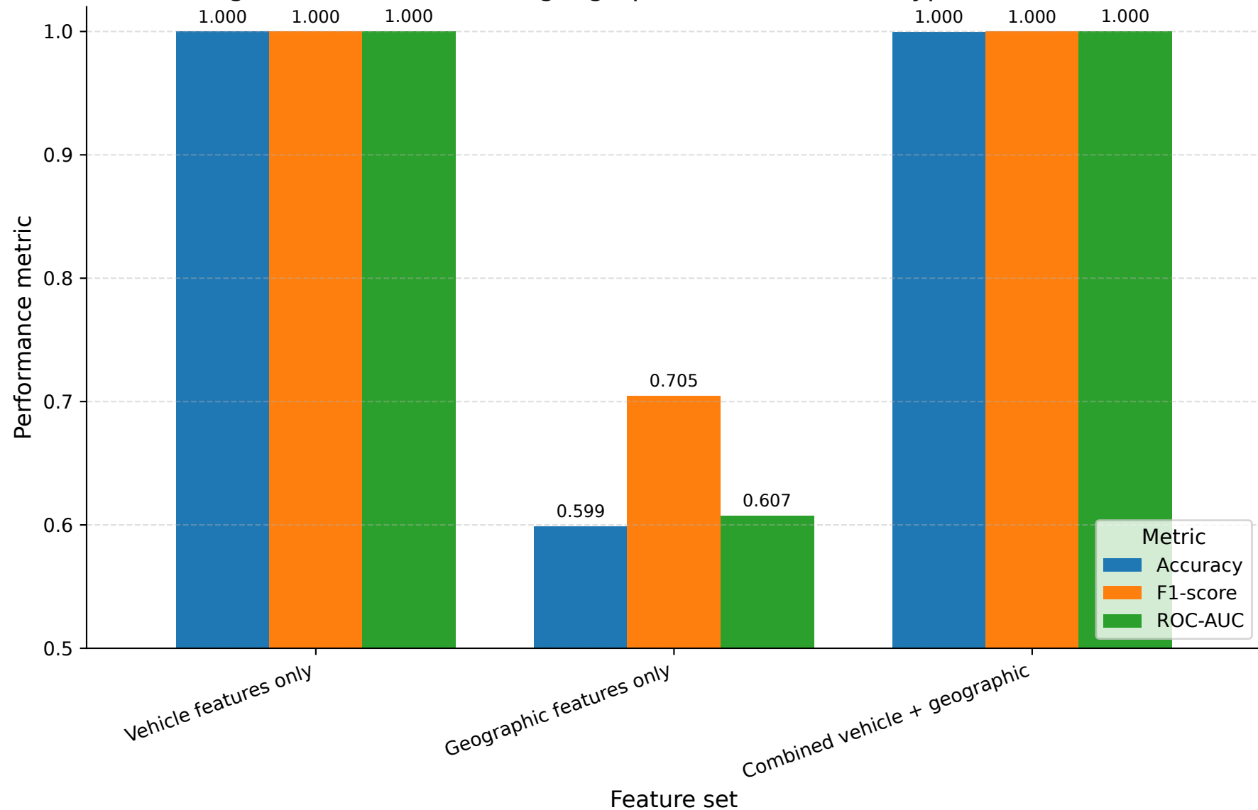
Figure 6. Added value of geographic variables in EV type classification
