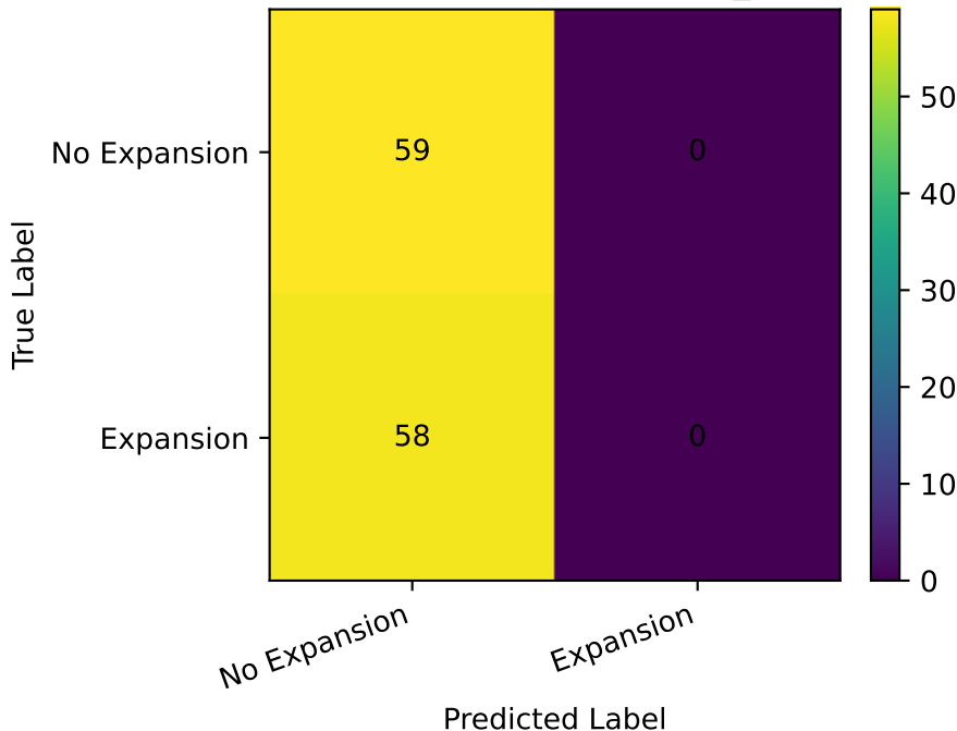
Confusion Matrix: Custom_CNN
