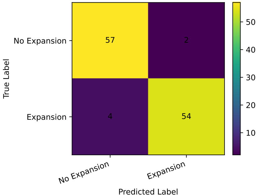
Confusion Matrix: ResNet50
