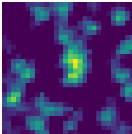
Grad-CAM Heatmap
