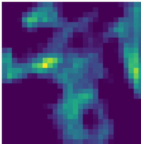
Grad-CAM Heatmap
