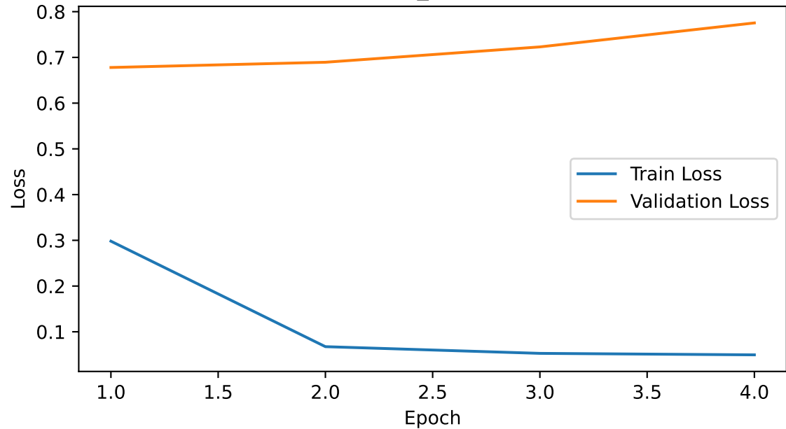
Custom_CNN Loss
