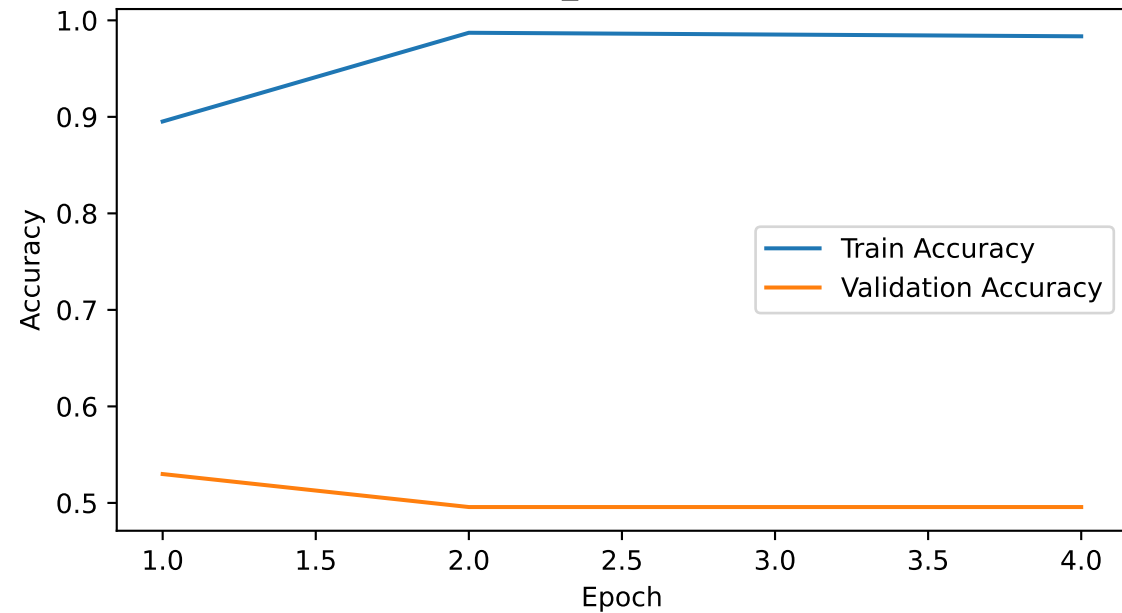
Custom_CNN Accuracy
