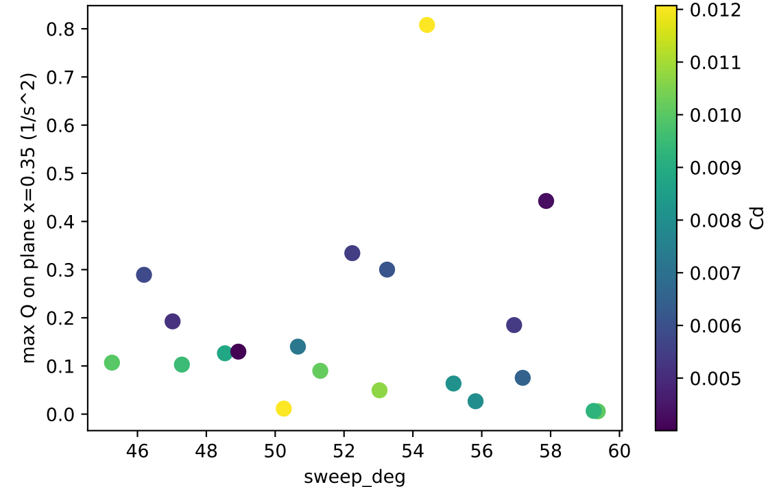
Vortex strength vs sweep (color=Cd)
