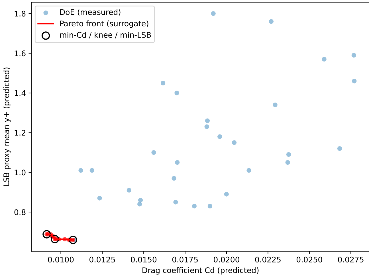
Tailfin planform Pareto front: drag vs LSB behavior
