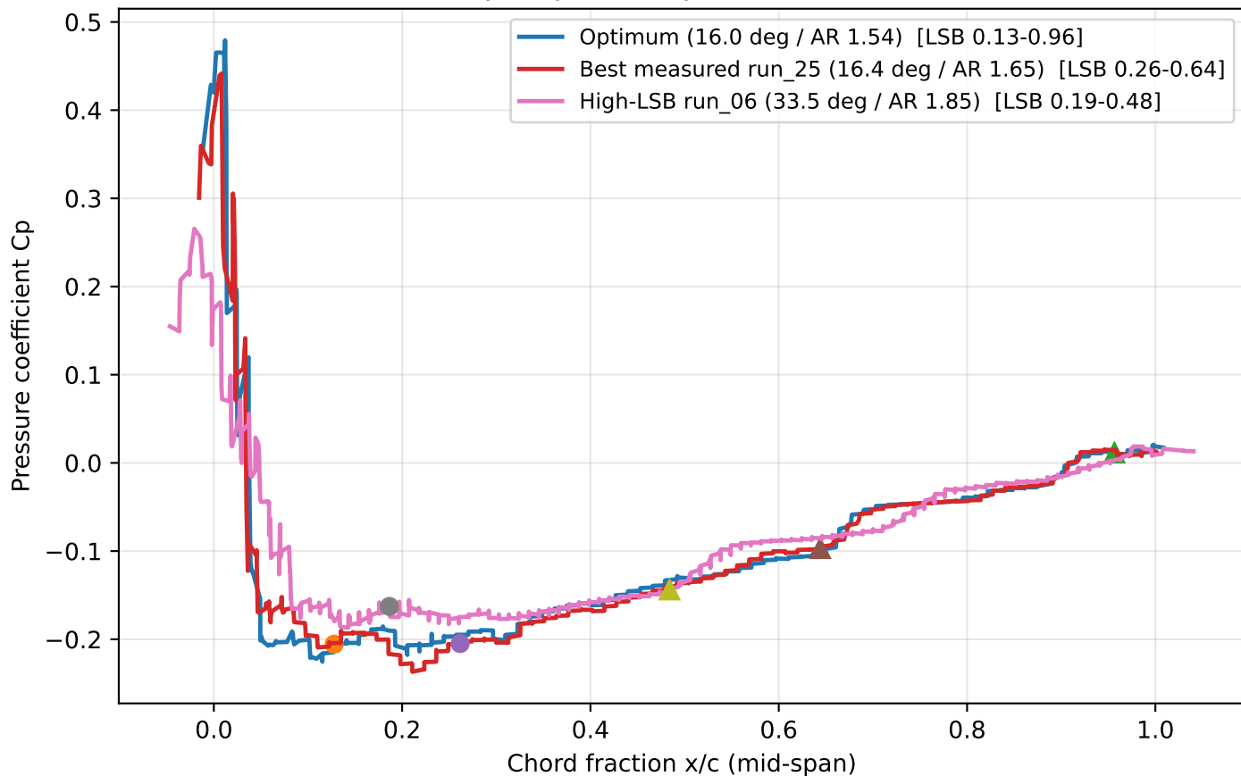
Chordwise C_p : separation plateau and reattachment
