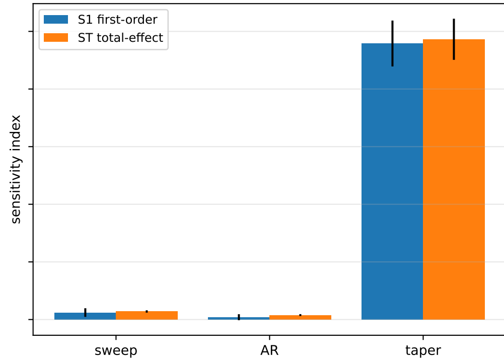
Sobol indices: lsb_mean
