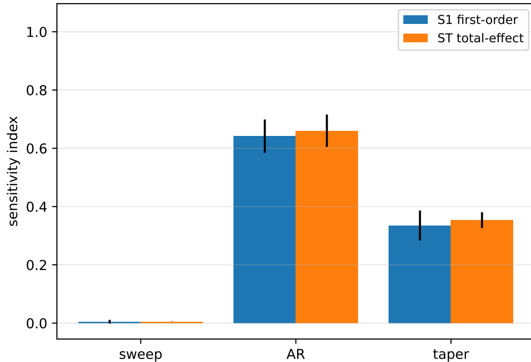
Sobol indices: Cd
