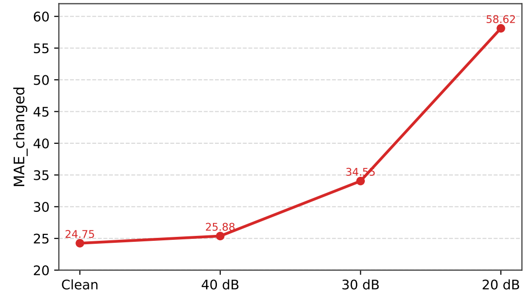
REG MAE_changed (lower is better)
