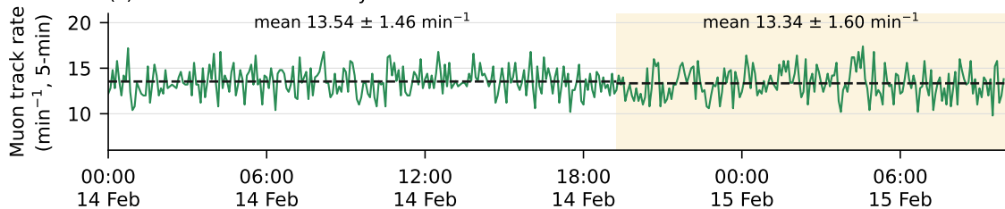
(c) Reconstructed three-layer track rate
