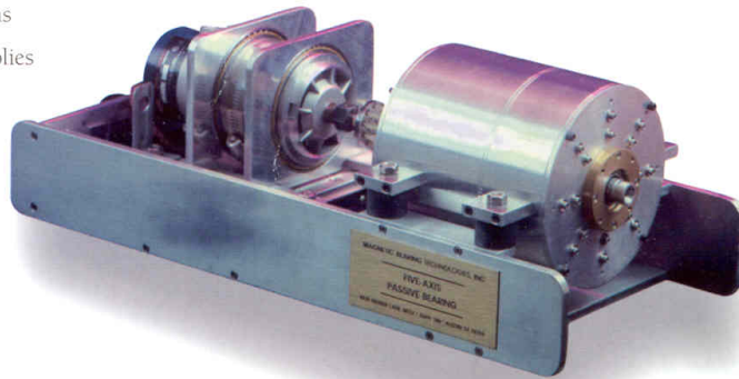
Demonstration Unit
