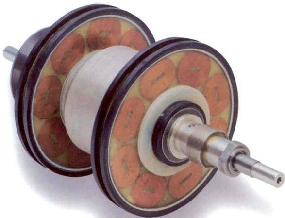
Prototype Rotor
