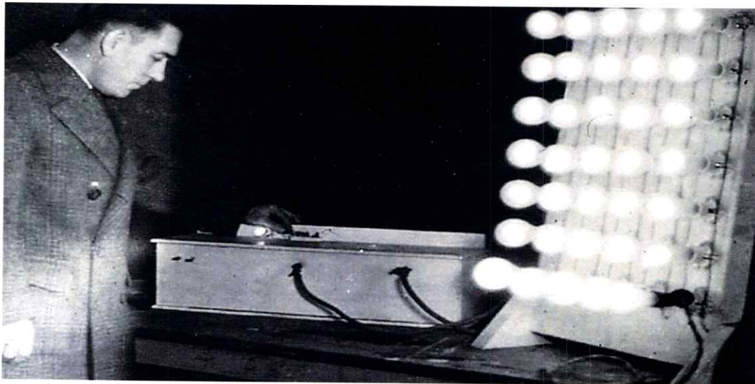
C. Todd lab photo of successful self-powering test of device in Feb. 1937. Unit was powering 35 100-watt lamps and a 1200-watt iron in this photo.
