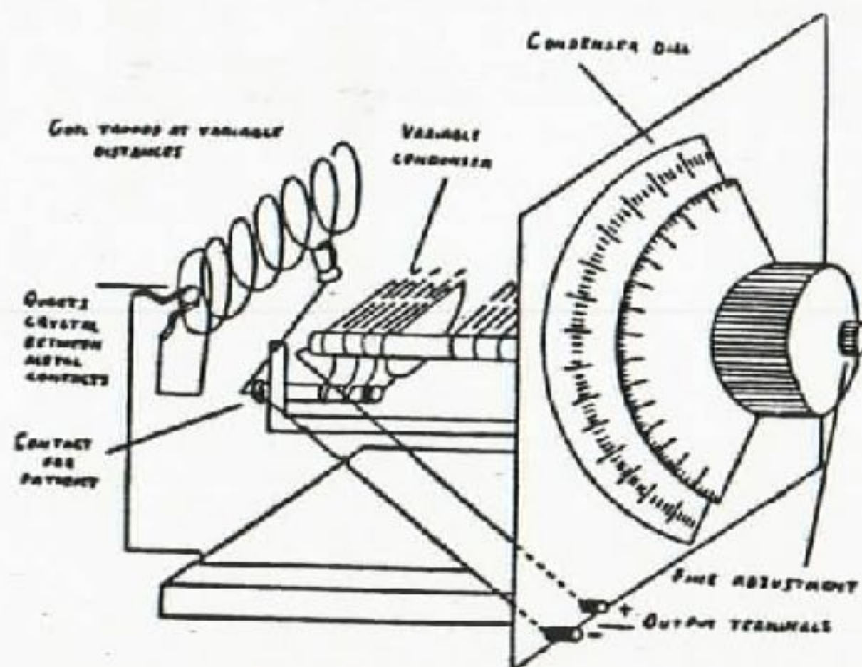
8. Crystal radio wave meter.
