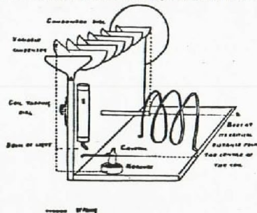
9. Mercury, crystal, coil and condenser combination.
